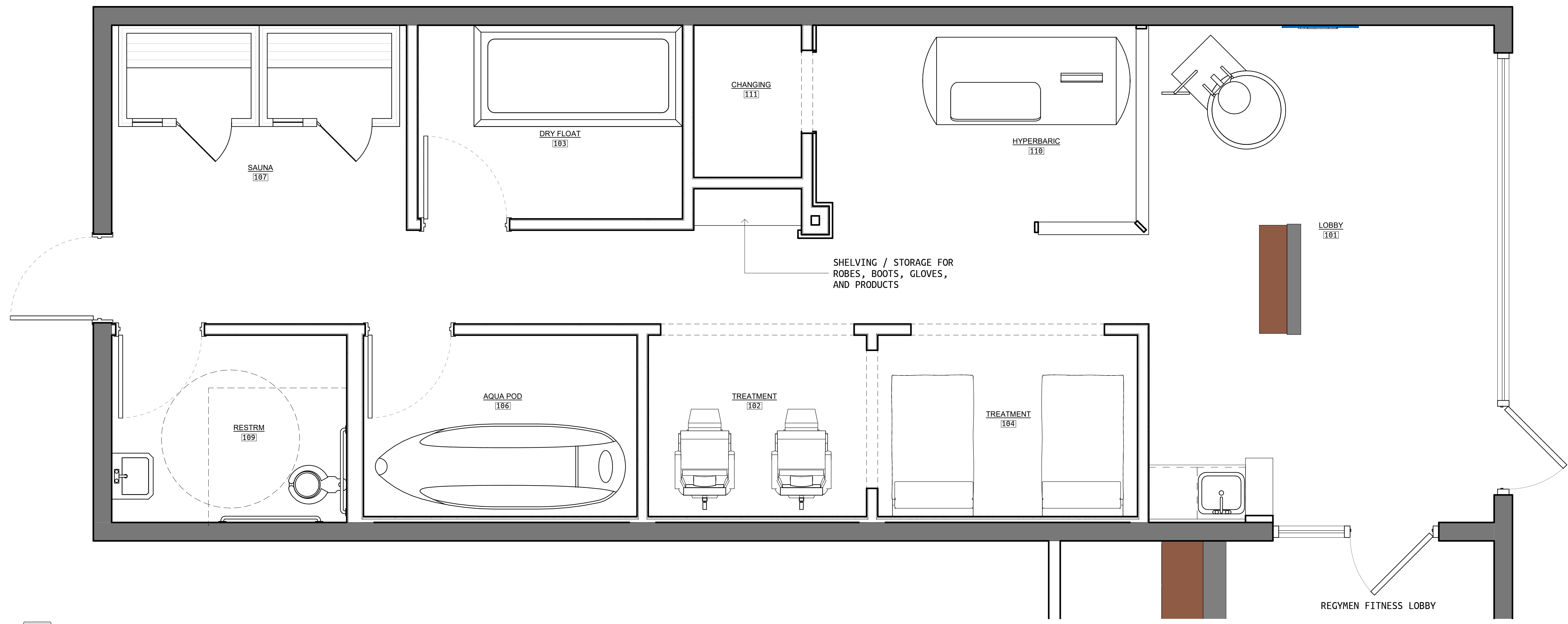
1 FLOOR PLAN 1/2" = 1'-0"
